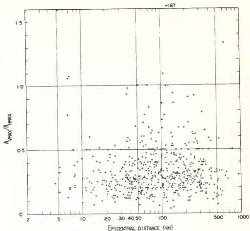
Fig. 3 Distribution of ratios of max. vertical acceleration to max. horizontal acceleration ( A_{vmax}/A_{hmax} ) to epicentral distance
